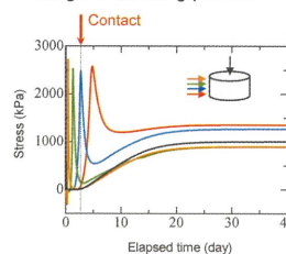
Change in swelling pressure
