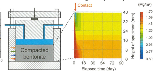
Change in dry density
