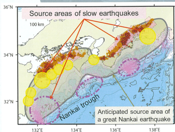
南海トラフ巨大地震想定震源域と各種スロー地震の発生場所 The anticipated source area of Nankai Trough megathrust earthquake and source areas of various slow earthquakes.
