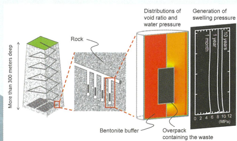
Change in swelling pressure
